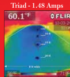
Triad - 1.48 Amps
